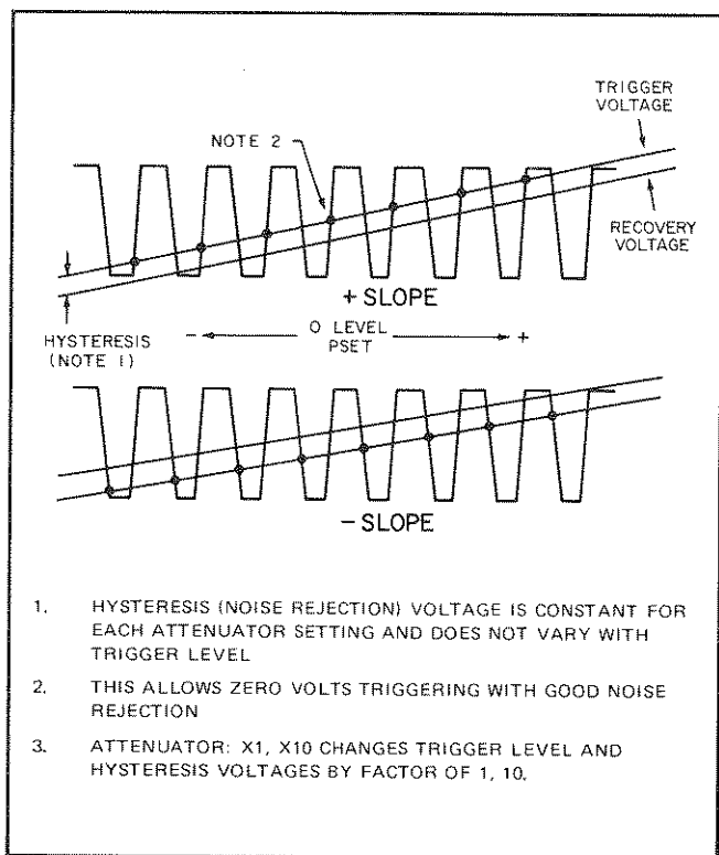
Figure 9H-3-1. Signal Conditioning Using Attenuator, Level and Slope Controls
