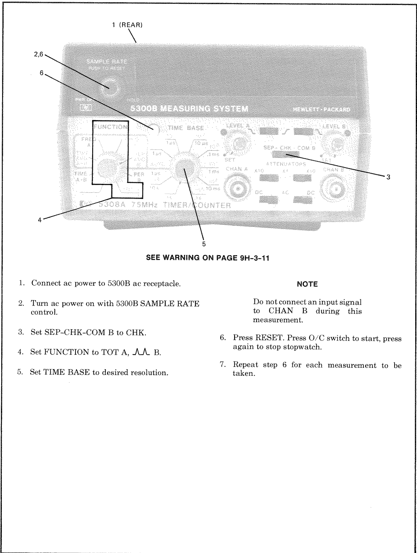
Figure 9H-3-12. Making Stopwatch Measurements
